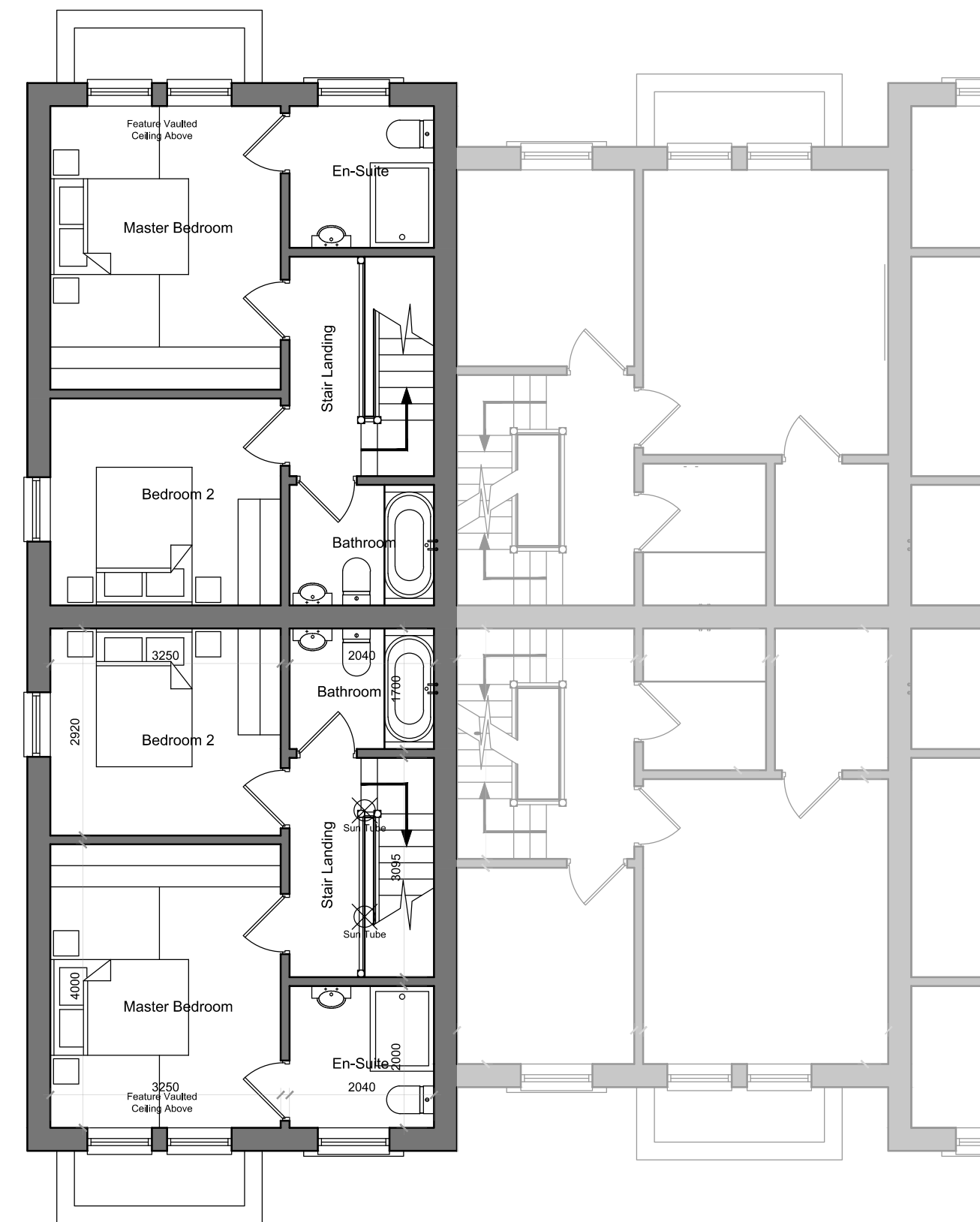
FIRST FLOOR
