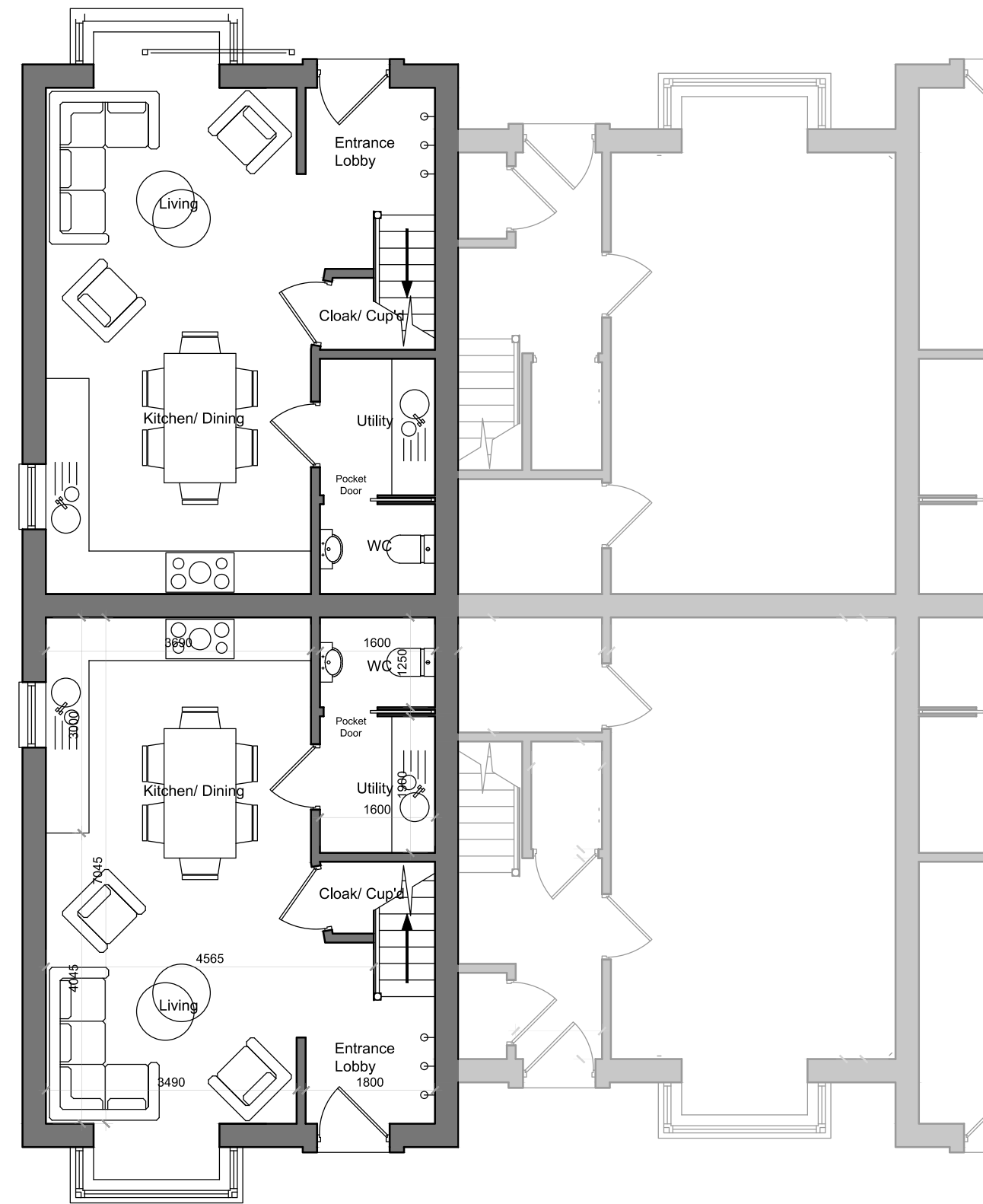
GROUND FLOOR
